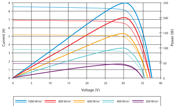
Current-Voltage & Power-Voltage Curve (250-20)
