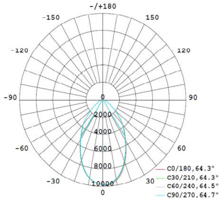
Average Beam Angle (50%) : 64.4 degree
